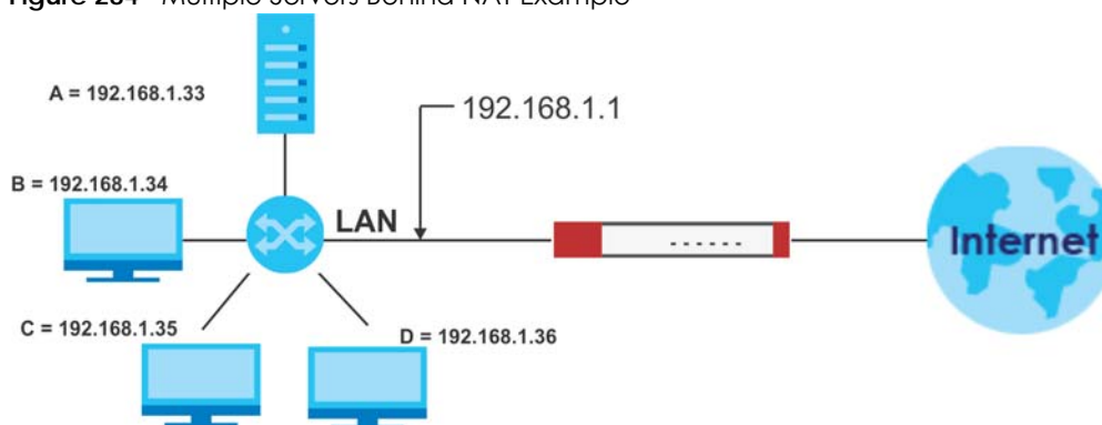
Figure 284 Multiple Servers Behind NAT Example
