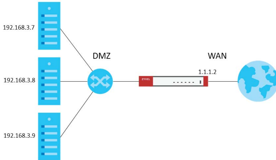
Figure 290 Virtual Server on the WAN- Example 1
