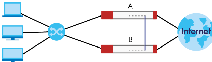
Figure 624 Device HA Pro
