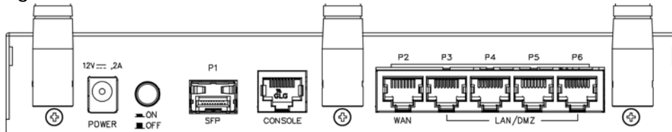
Figure 66 ATP100W Rear Panel
