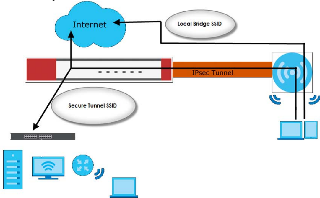
Figure 311 AP Using Secure Tunnel SSID Profile
