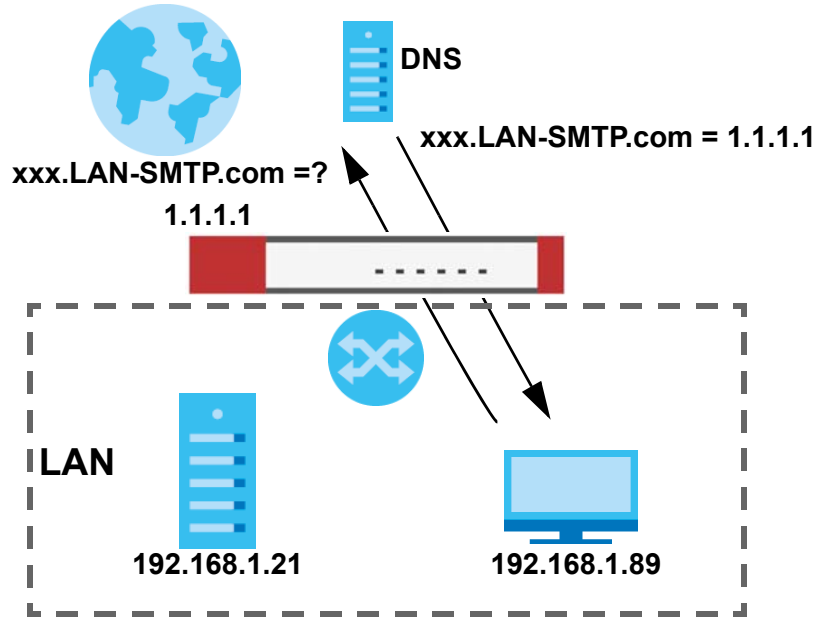
Figure 287 LAN Computer Queries a Public DNS Server
