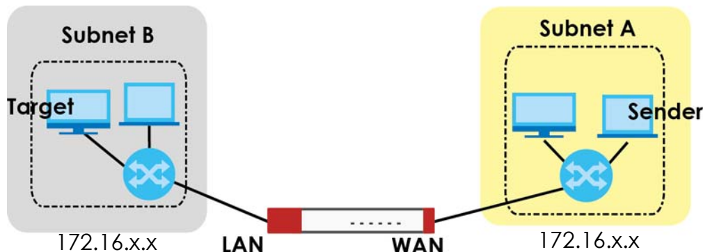
Figure 227 Proxy ARP
