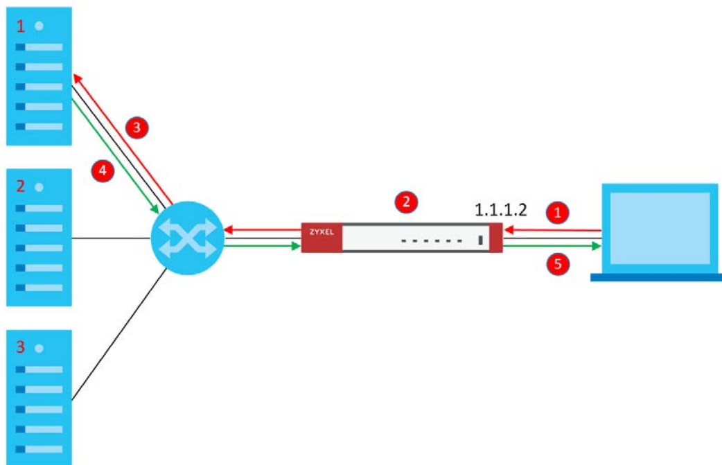
Figure 292 Load Balancing Process
