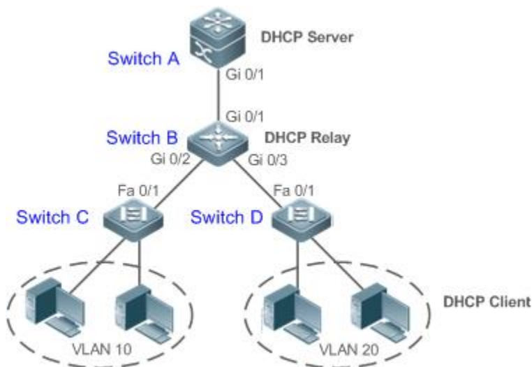
Figure 4-4 DHCP Relay
