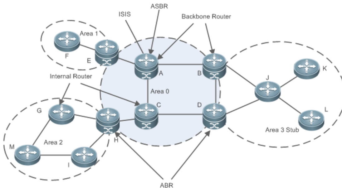
Figure 5-3 Division of the OSPF Areas
