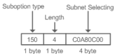
Figure 4-13 Subnet-Selection
