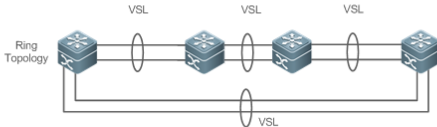
Figure 8-9 Ring Topology
