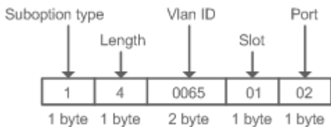
Figure 4-8 Agent Remote ID
