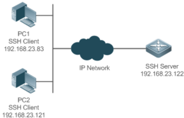
Figure 15-2 Networking Topology of SSH Local Line Password Authentication
