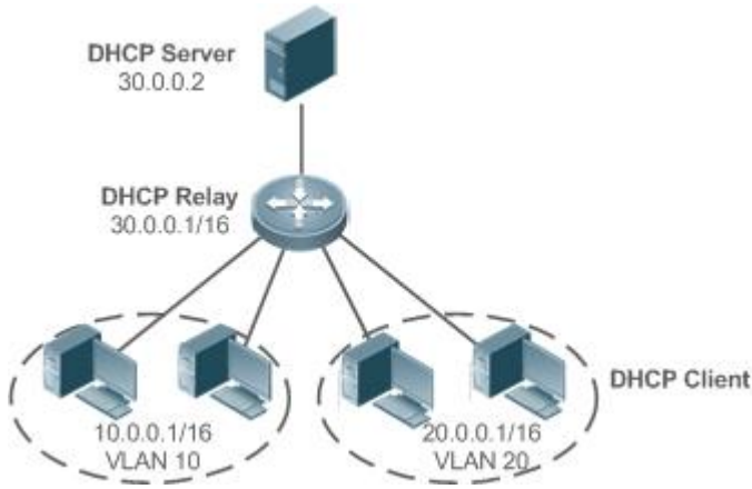
Figure 4-6 DHCP Relay Scenario
