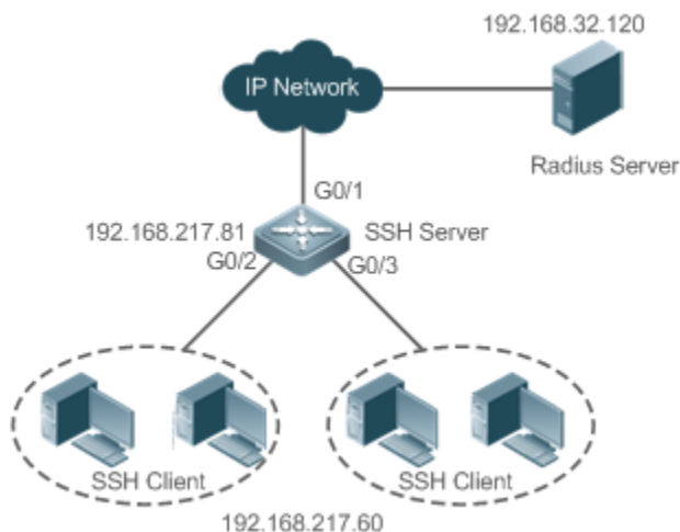
Figure 15-3 Networking Topology of SSH AAA Authentication
