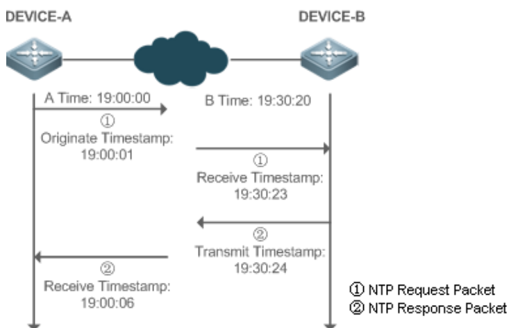
Figure 13-3 Working Principle of SNTP
