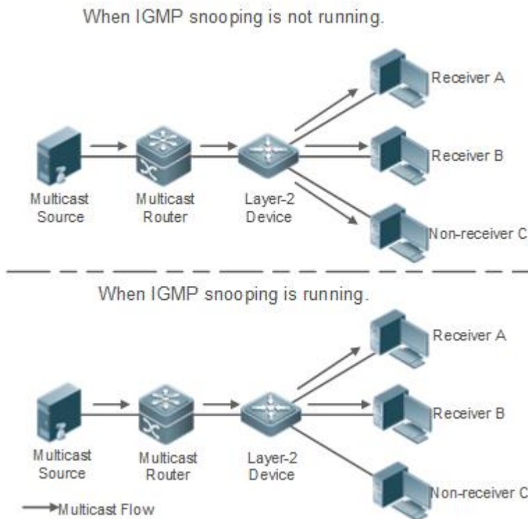
Figure 11-1 Networking Topology of IP Multicast Forwarding within the VLAN Before and After IGMP Snooping Is Run on the Layer-2 Device
