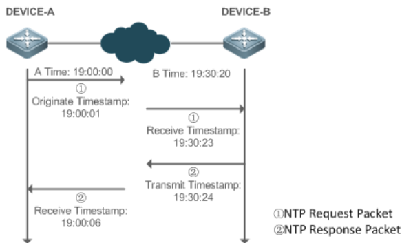
Figure 12-4 Working Principle of NTP
