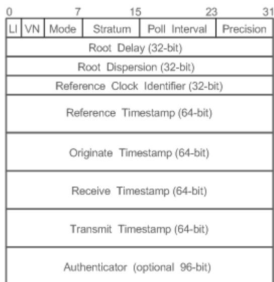
Figure 13-2 Format of an SNTP Time Synchronization Packet
