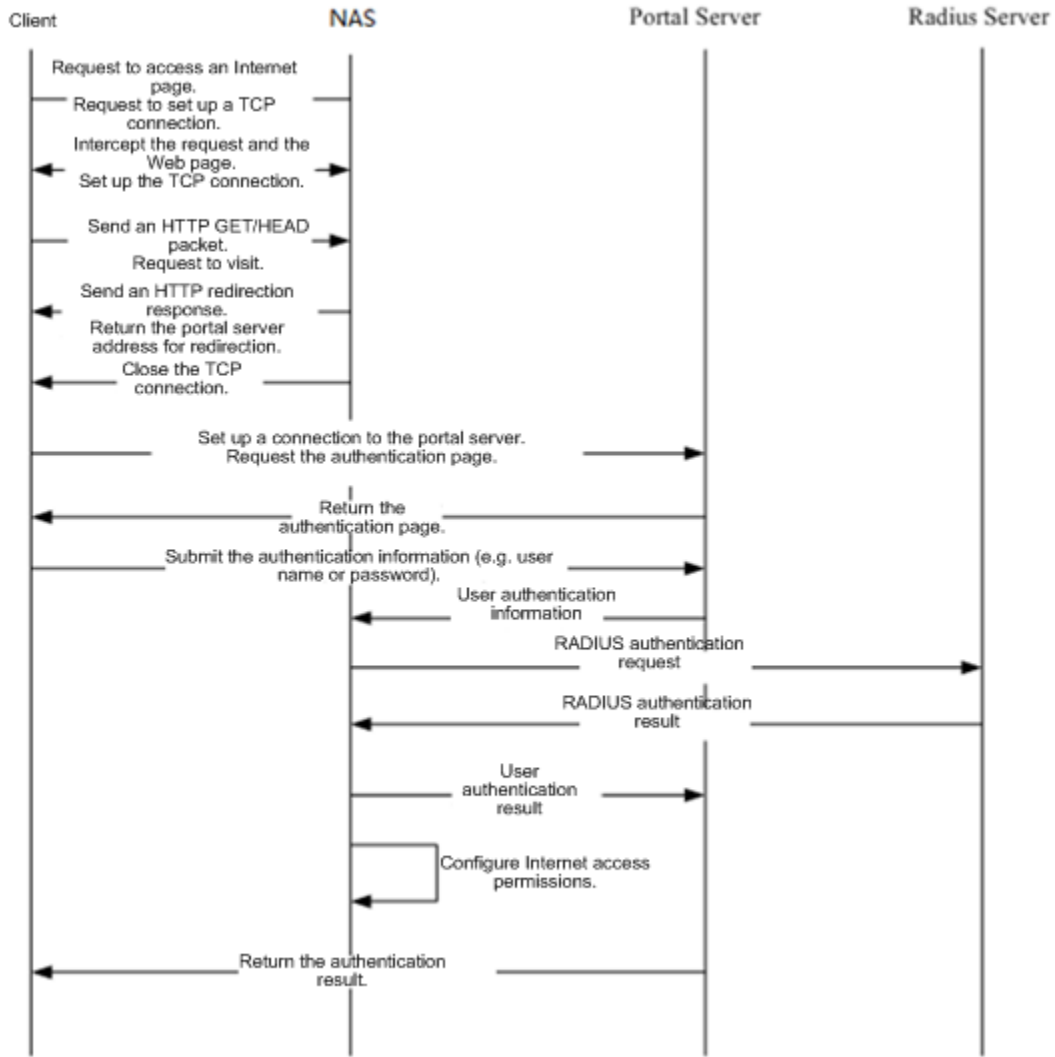
Figure 1-4 Flowchart of Ruijie Second-Generation Web Authentication
