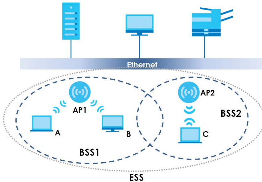
Figure 139 Infrastructure WLAN
