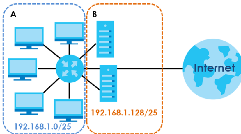
Figure 127 Subnetting Example: After Subnetting
