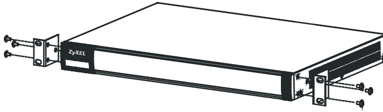
Figure 71 Attach Brackets
