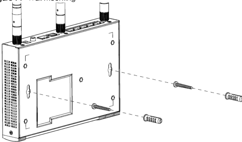
Figure 74 Wall Mounting
