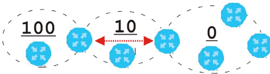
Figure 273 OSPF: Virtual Link
