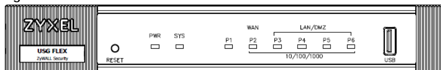
Figure 61 USG FLEX 100W Front Panel
