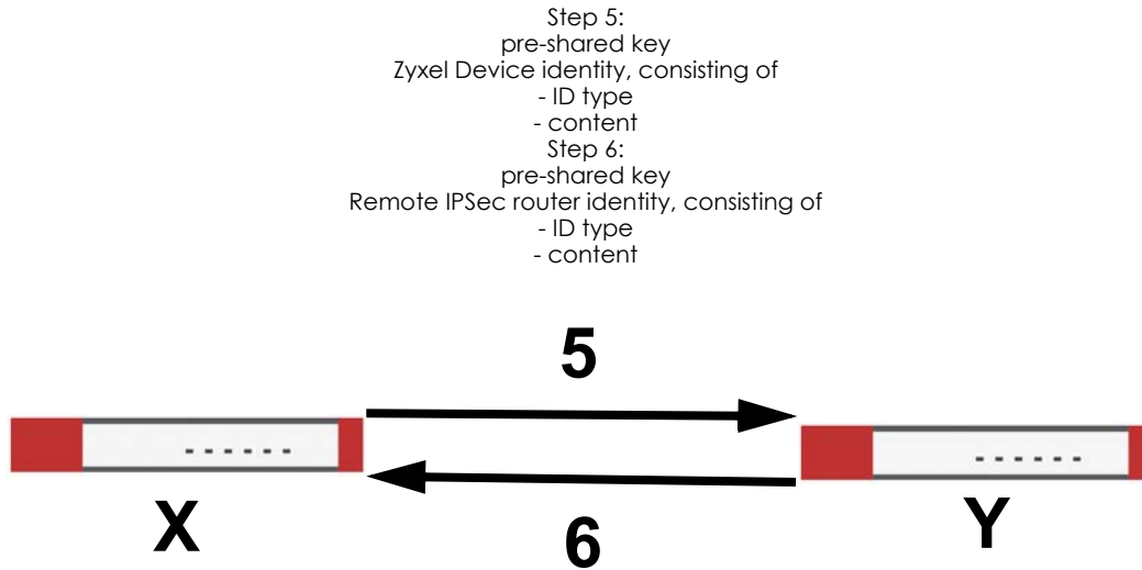
Figure 379 IKE SA: Main Negotiation Mode, Steps 5 - 6: Authentication (continued)
