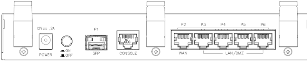
Figure 67 USG FLEX 200 Rear Panel
