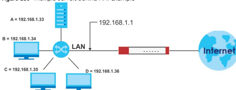
Figure 285 Multiple Servers Behind NAT Example
