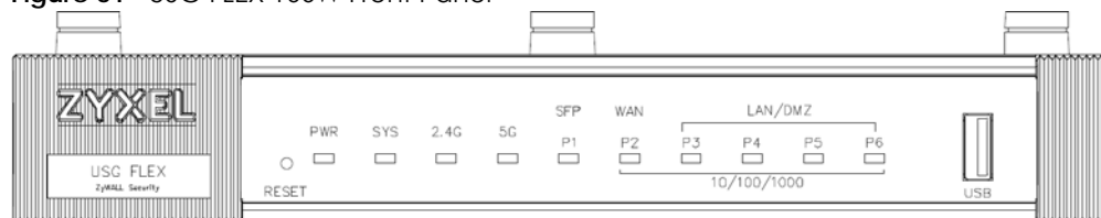
Figure 61 USG FLEX 100W Front Panel
