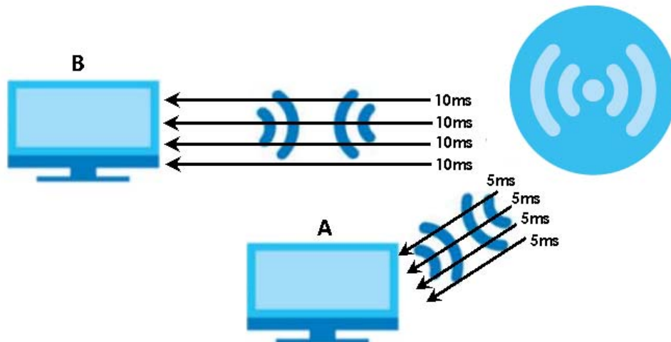
Figure 308 Airtime Fairness Example-Disabled
