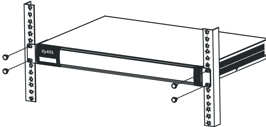
Figure 72 Mount on Rack
