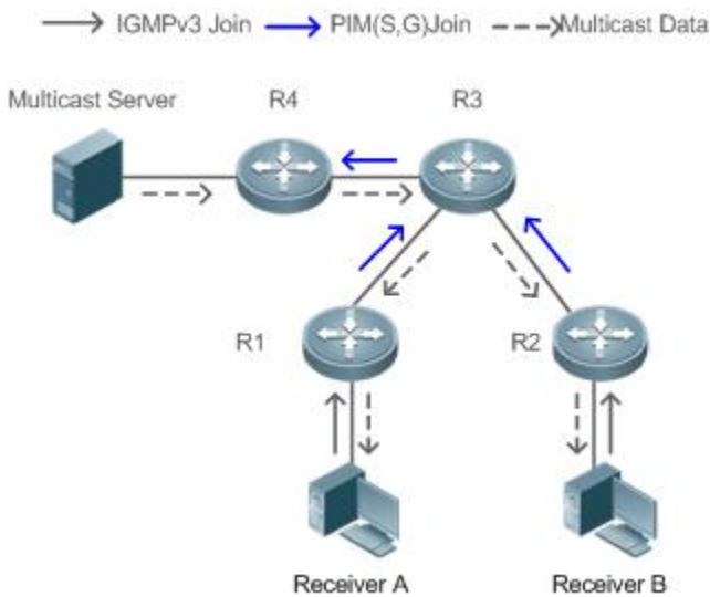
Figure 6-4 SSM Model
