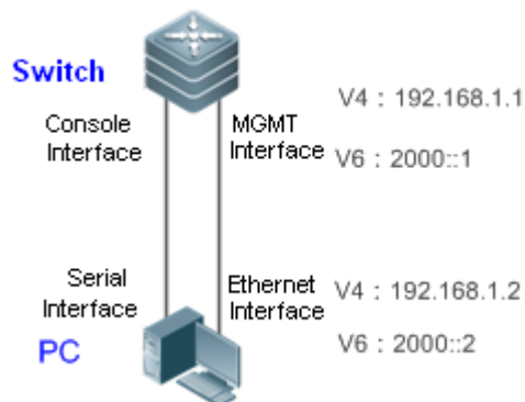
Figure 14-3 Network Login Management
