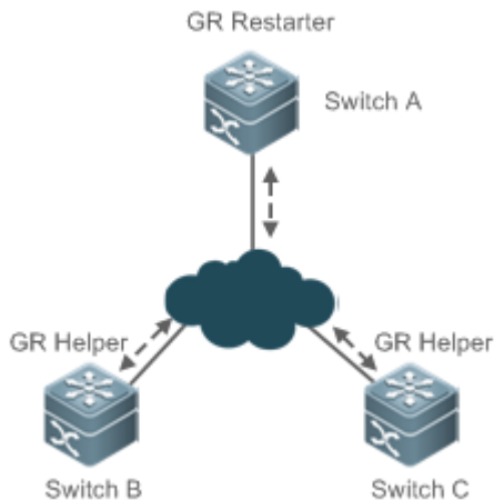
Figure 6-17 GR Completion
