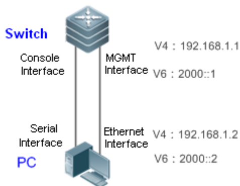
Figure 14-1 Network Management Tool
