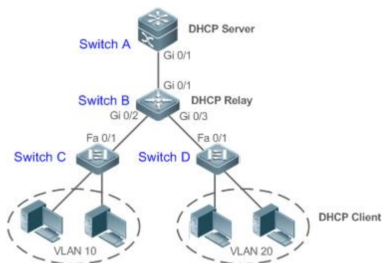
Figure 4-4 DHCP Relay
