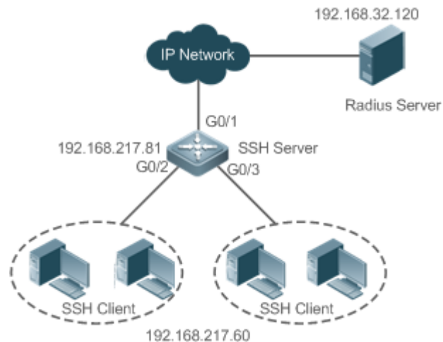
Figure 10-3 Networking Topology of SSH AAA Authentication
