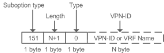
Figure 4-12 VPN-ID
