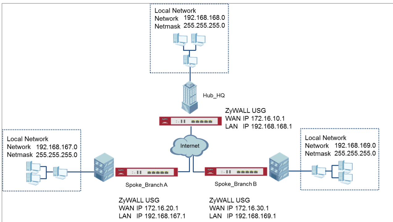
ZyWALL/USG Hub-and-Spoke VPN Example
