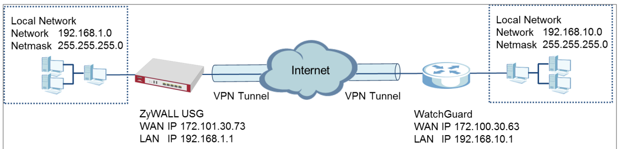
ZyWALL Site-to-site IPSec VPN with WatchGuard Connected
