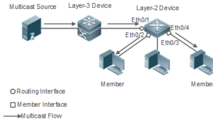
Figure 13-5 Networking Topology of Two IGMP Snooping Ports
