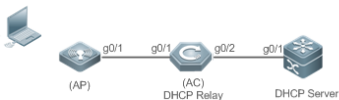
Figure 4-6 DHCP Server Network Topology
