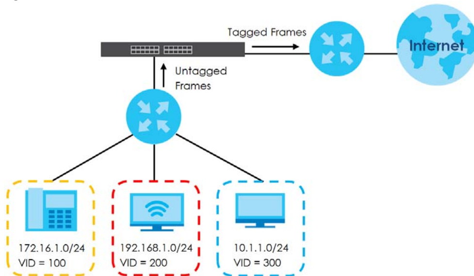
Figure 321 Subnet Based VLAN Application Example
