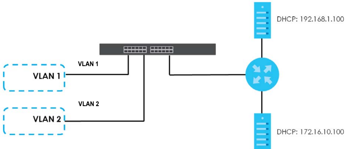
Figure 375 DHCP Relay for Two VLANs
