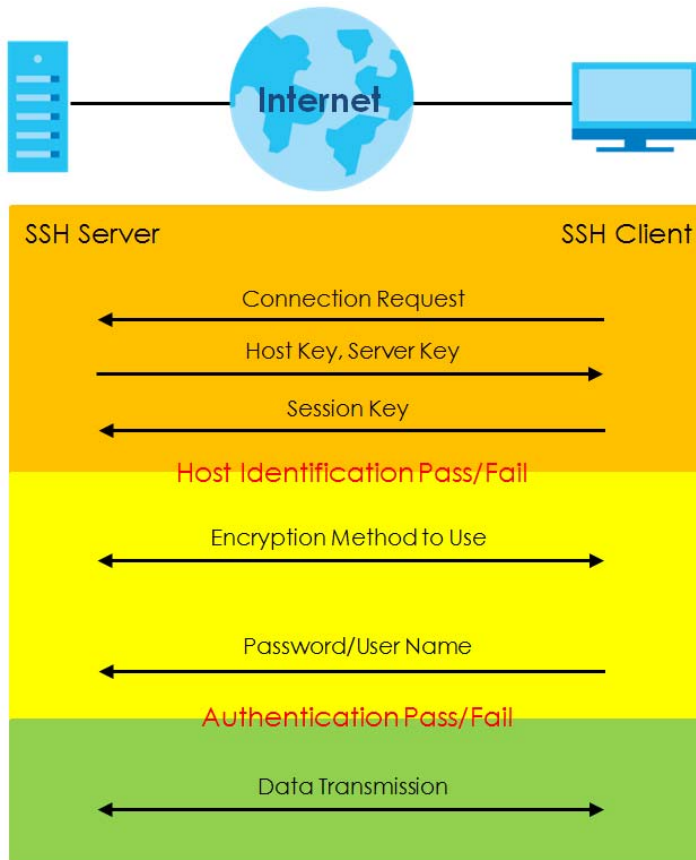
Figure 443 How SSH Works
