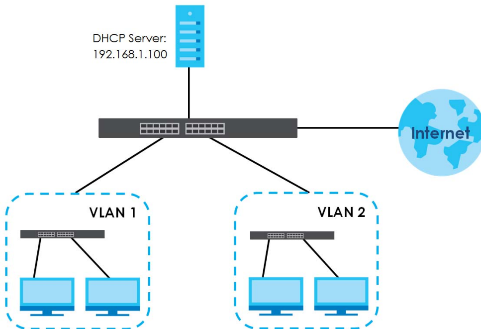
Figure 366 DHCP Smart Relay Network Example
