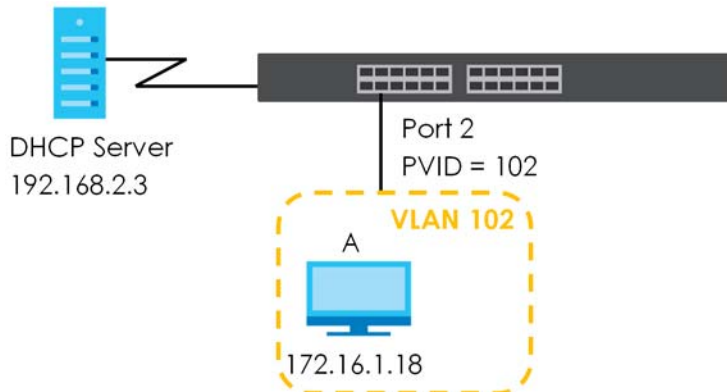
Figure 56 Tutorial: DHCP Relay Scenario
