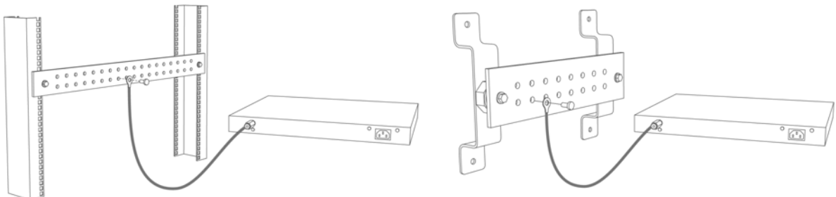
Figure 22 Attach Ground Cable to Grounding Bar or On-site Grounding Terminal
