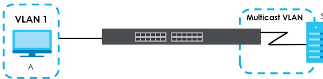
Figure 220 MVR Multicast Television Example
