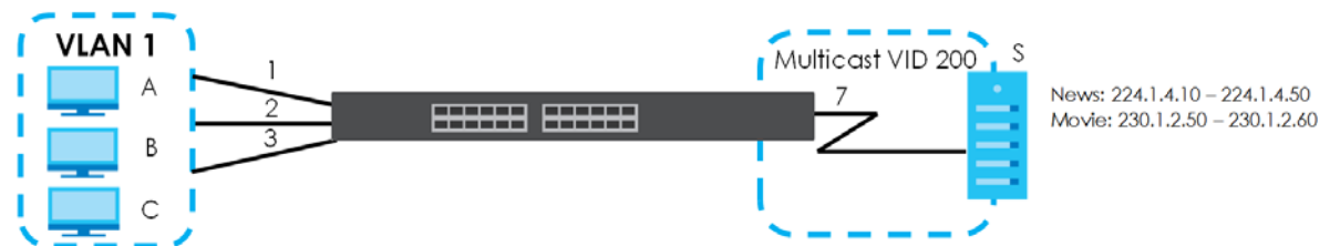
Figure 245 MVR Configuration Example
