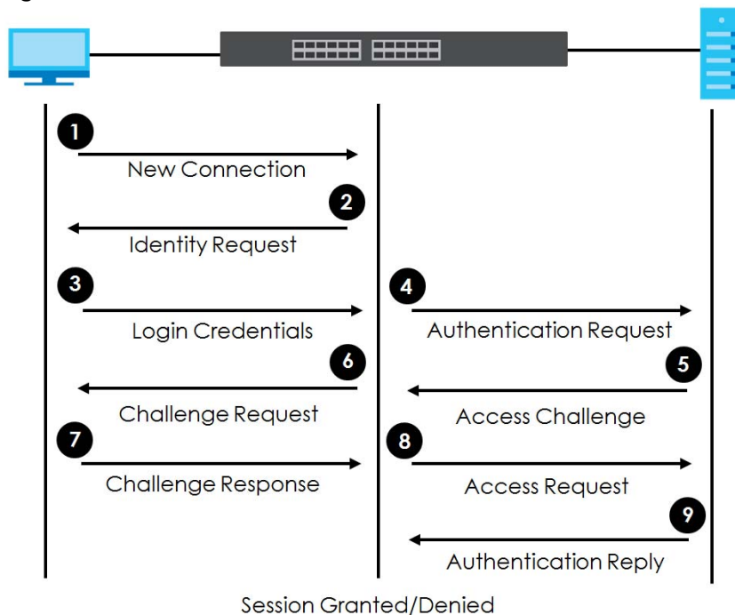
Figure 510 IEEE 802.1x Authentication Process
