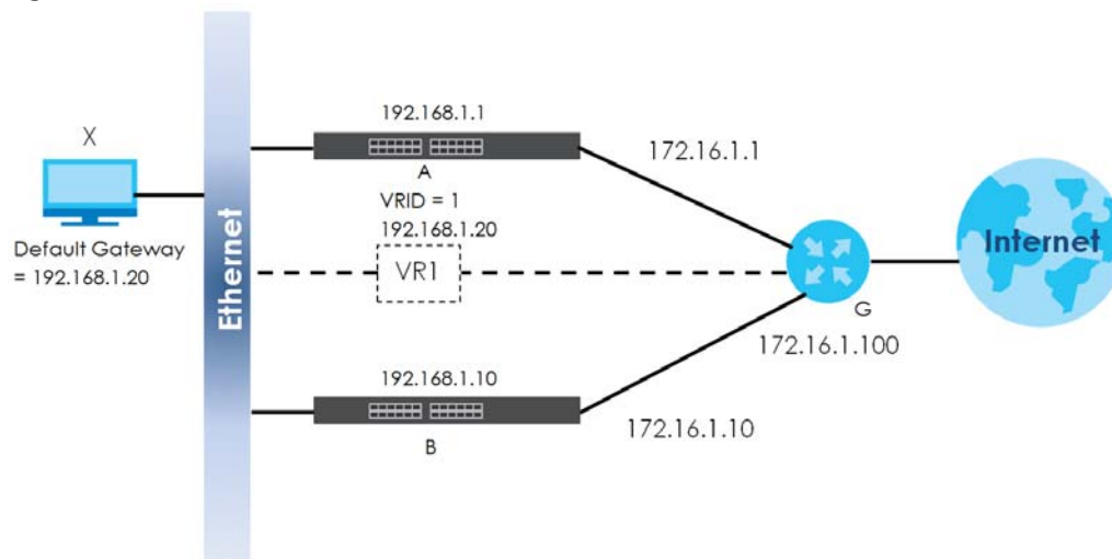
Figure 425 VRRP Configuration Example: One Virtual Router Network
