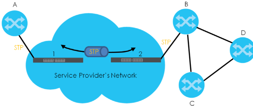
Figure 195 L2PT Network Example
