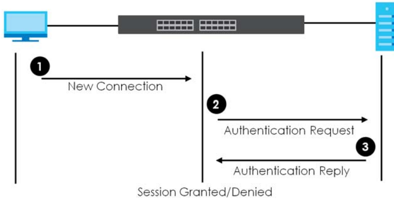
Figure 511 MAC Authentication Process
