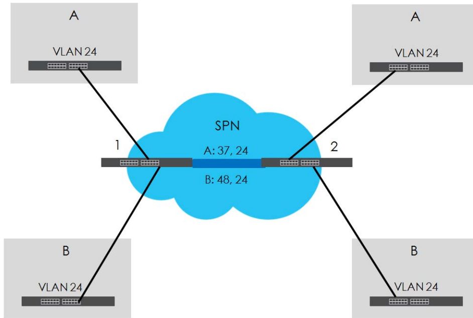
Figure 346 VLAN Stacking Example
