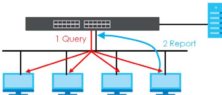
Figure 389 IGMP Version 1 Example
