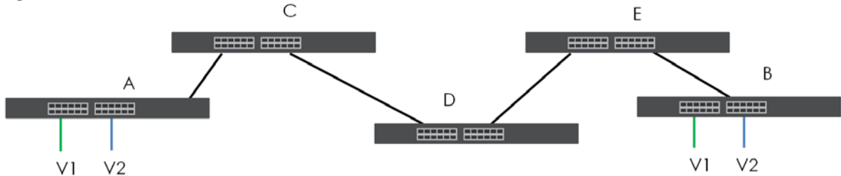
Figure 583 Port VLAN Trunking
