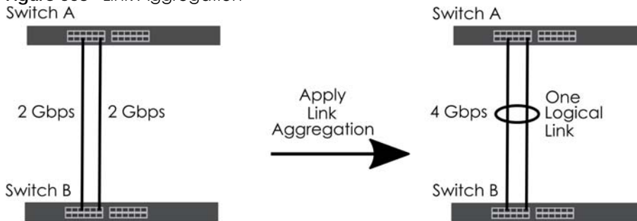
Figure 568 Link Aggregation
