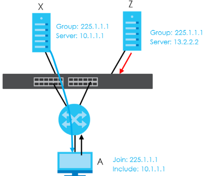
Figure 391 IGMP Version 3 Example
