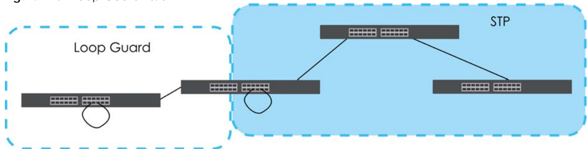
Figure 198 Loop Guard vs. STP
