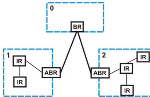
Figure 398 OSPF Network Example
