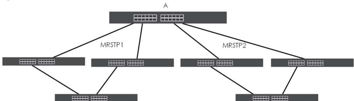
Figure 280 MRSTP Network Example
