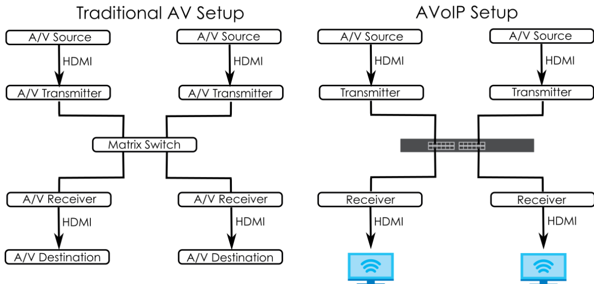
Figure 4 Comparison Between Traditional AV and AVoIP Setups
