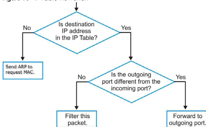
Figure 70 IP Table Flowchart
