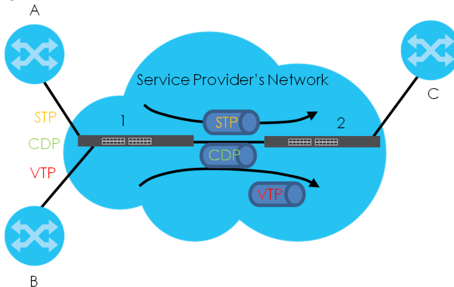
Figure 194 Layer 2 Protocol Tunneling Network Scenario
