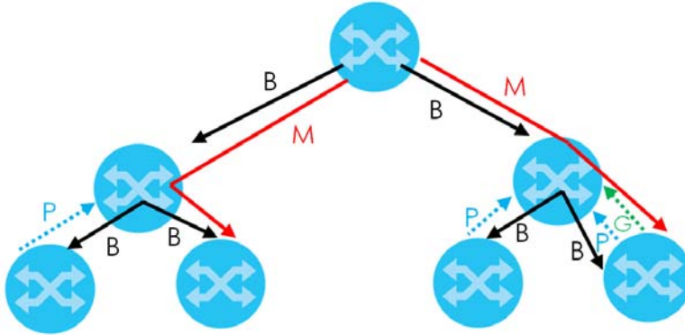
Figure 386 How DVMRP Works
