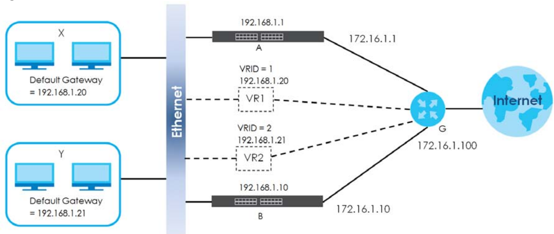
Figure 430 VRRP Configuration Example: Two Virtual Router Network
