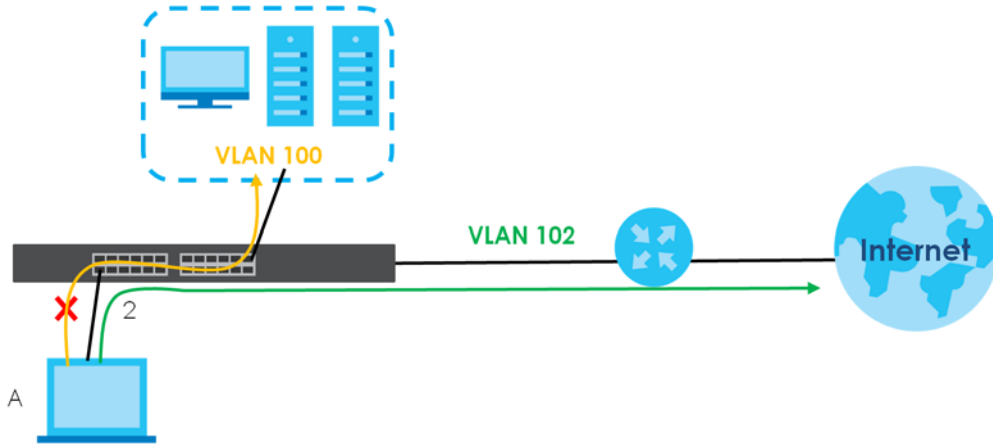
Figure 516 Guest VLAN Example
