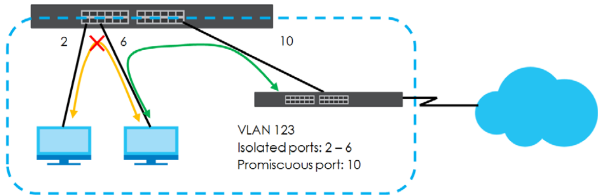
Figure 337 VLAN Isolation Example
