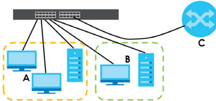
Figure 324 Protocol Based VLAN Application Example
