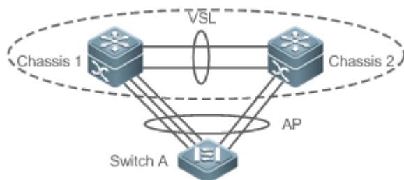
Figure 5-15 Cross-device aggregation port
