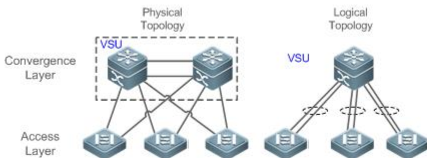
Figure 5-5 Convergence layer VSU
