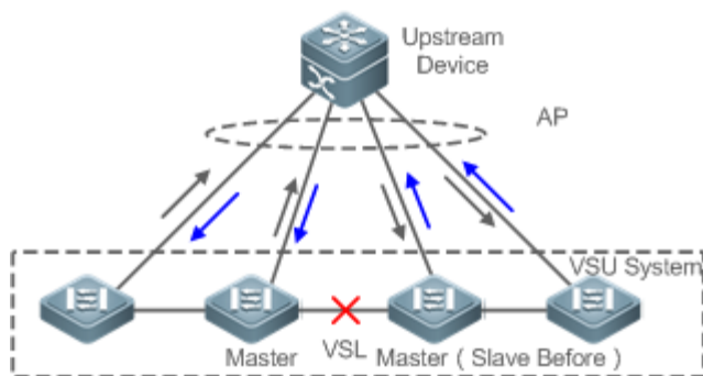
Figure 5-14 MAD based on upstream and downstream devices
