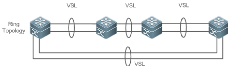
Figure 5-9 Ring Topology
