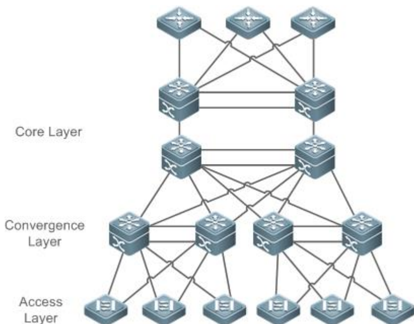
Figure 5-1 Traditional Network Architecture
