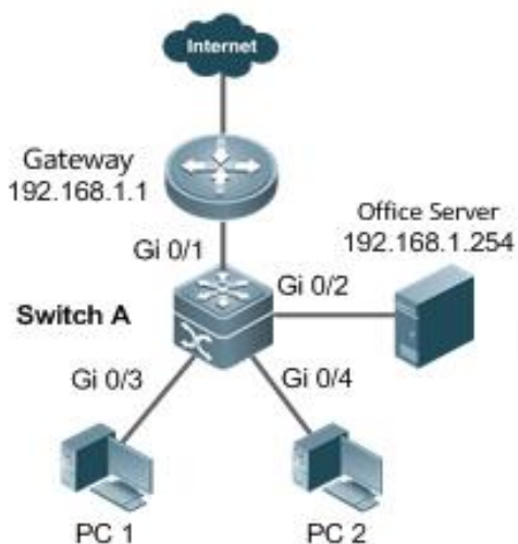
Figure 19-1 Typical Topology of Gateway-targeted ARP Spoofing Prevention
