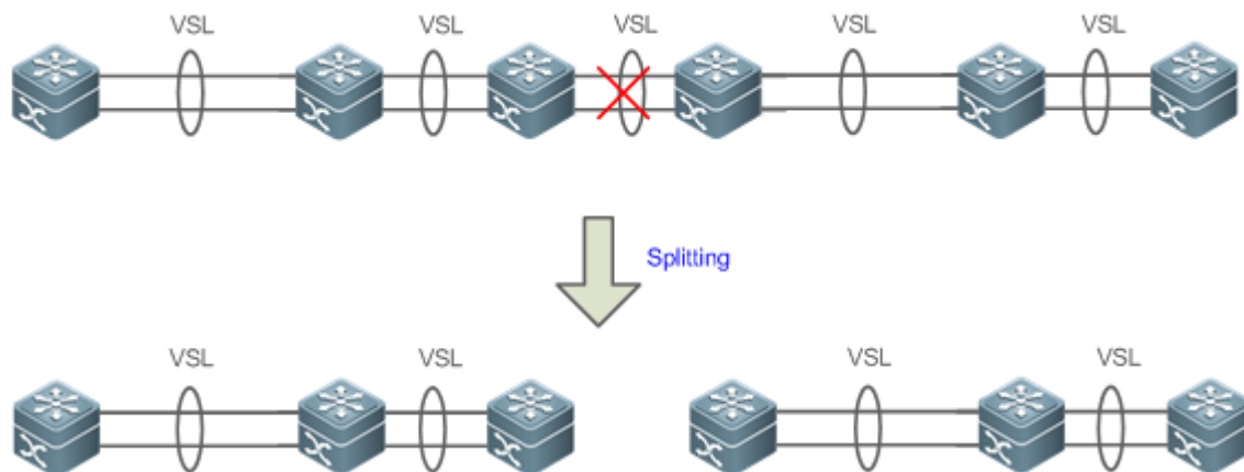
Figure 5-11 Topology splitting
