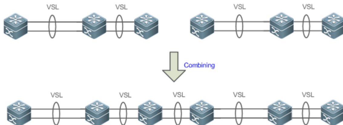
Figure 5-12 Topology combining
