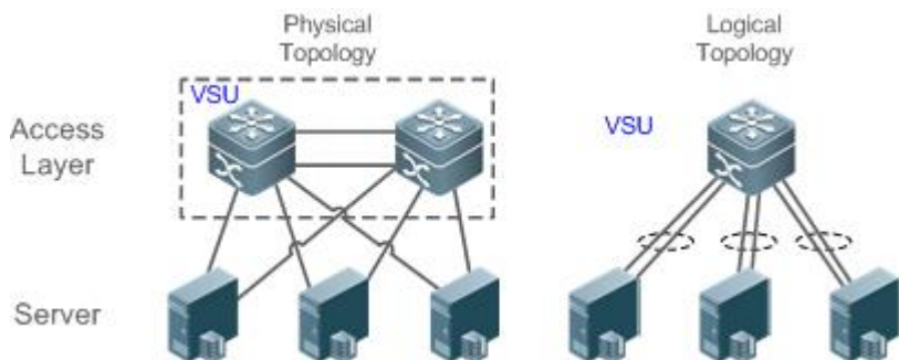
Figure 5-6 Access layer VSU
