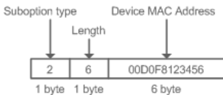
Figure 4-8 Agent Remote ID
