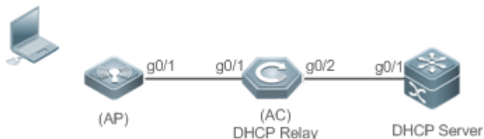
Figure 4-3 DHCP Relay
