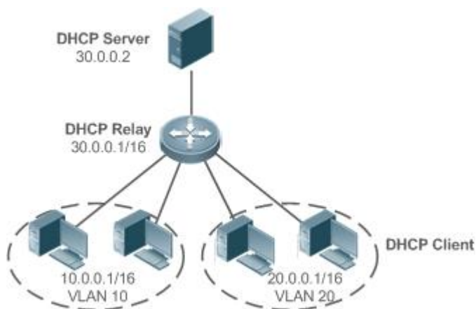
Figure 4-6 DHCP Relay Scenario
