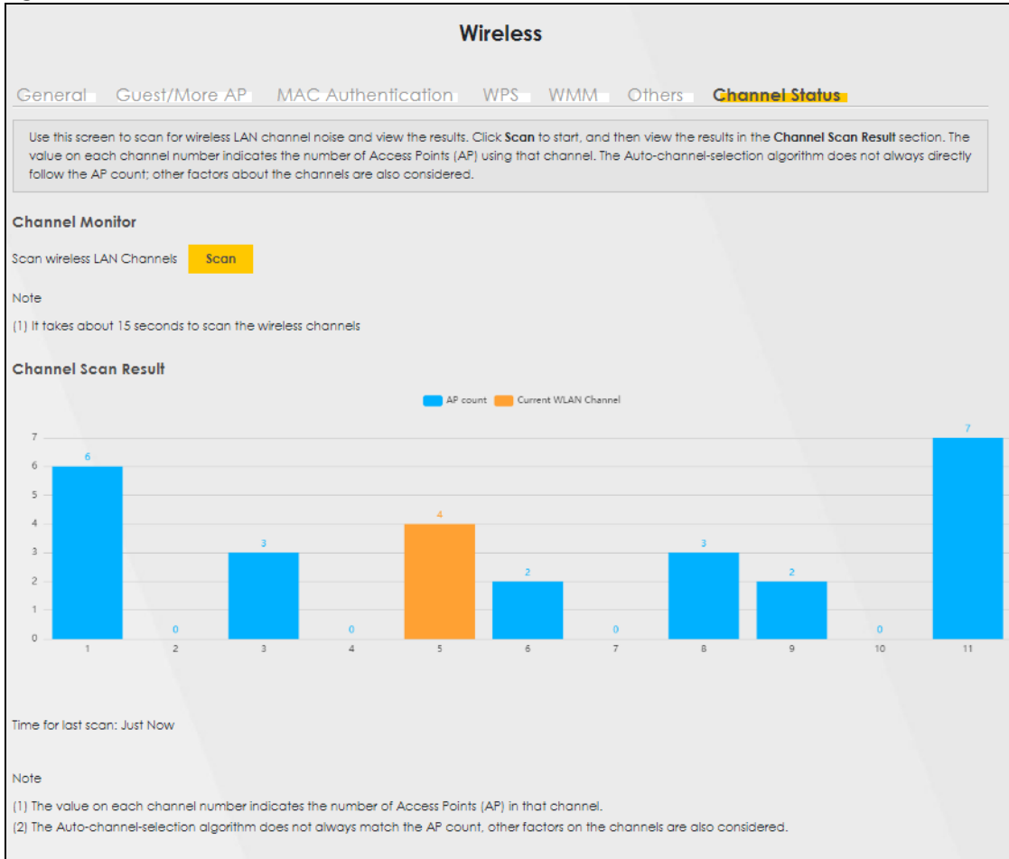
Figure 108 Network Setting &gt; Wireless &gt; Channel Status
