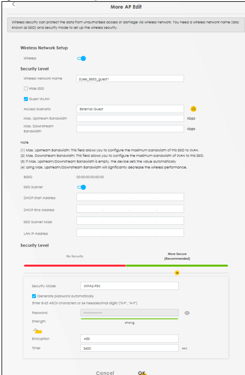
Figure 103 Network Setting > Wireless > Guest/More AP > Edit
