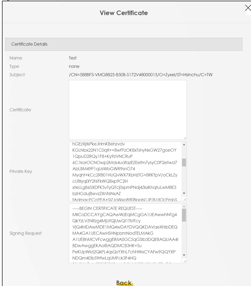
Figure 210 Security > Certificates > Local Certificates: View Certificate
