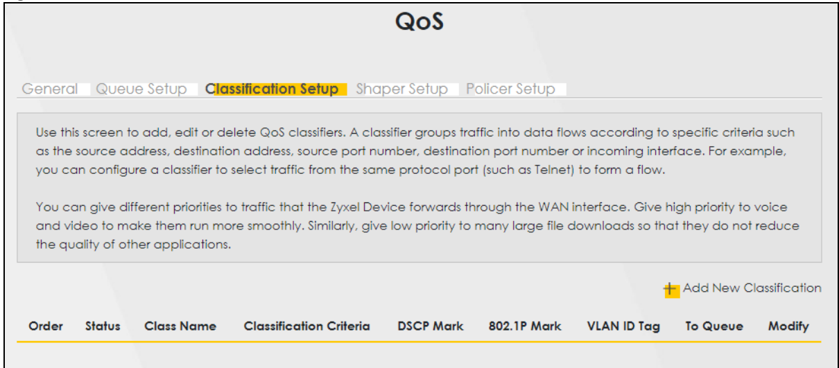
Figure 150 Network Setting > QoS > Classification Setup
