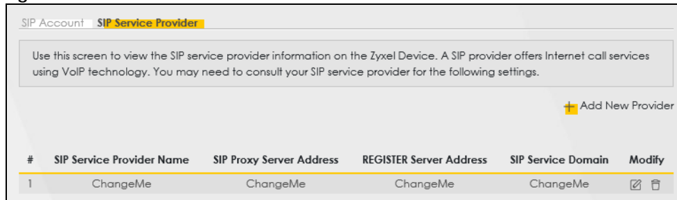
Figure 219 VoIP &gt; SIP &gt; SIP Service Provider
