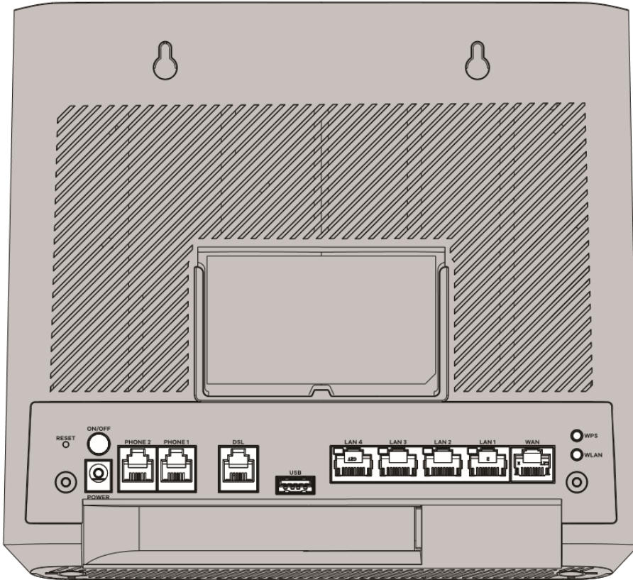
Figure 24 DX5301-B2 / DX5301-B3
