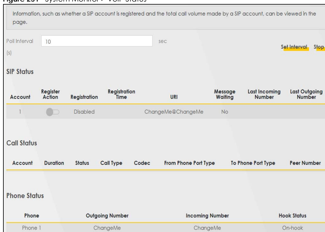
Figure 231 System Monitor > VoIP Status
