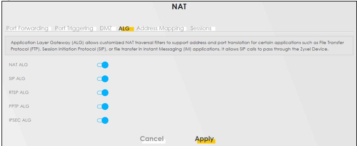
Figure 163 Network Setting > NAT > ALG
