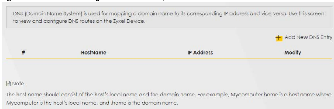
Figure 170 Network Setting > DNS > DNS Entry
