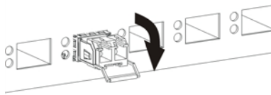
Figure 39 Transceiver Removal Example
