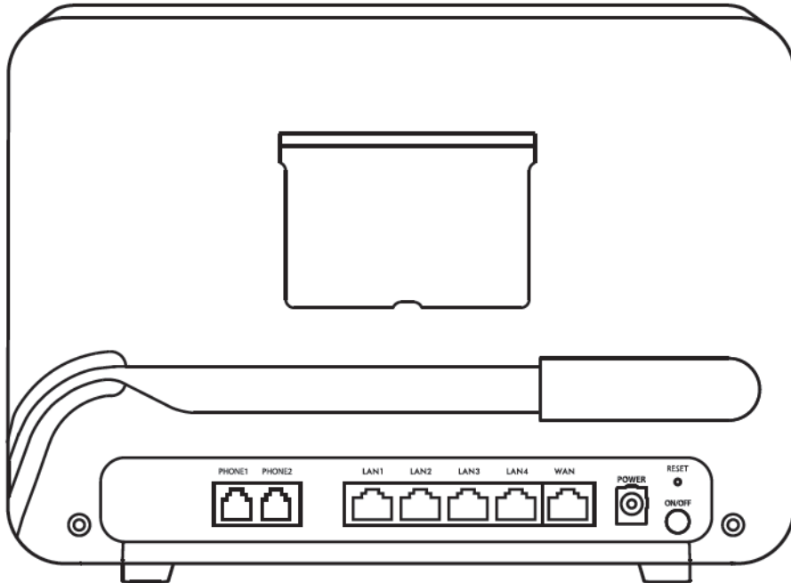
Figure 30 EX5401-B0
