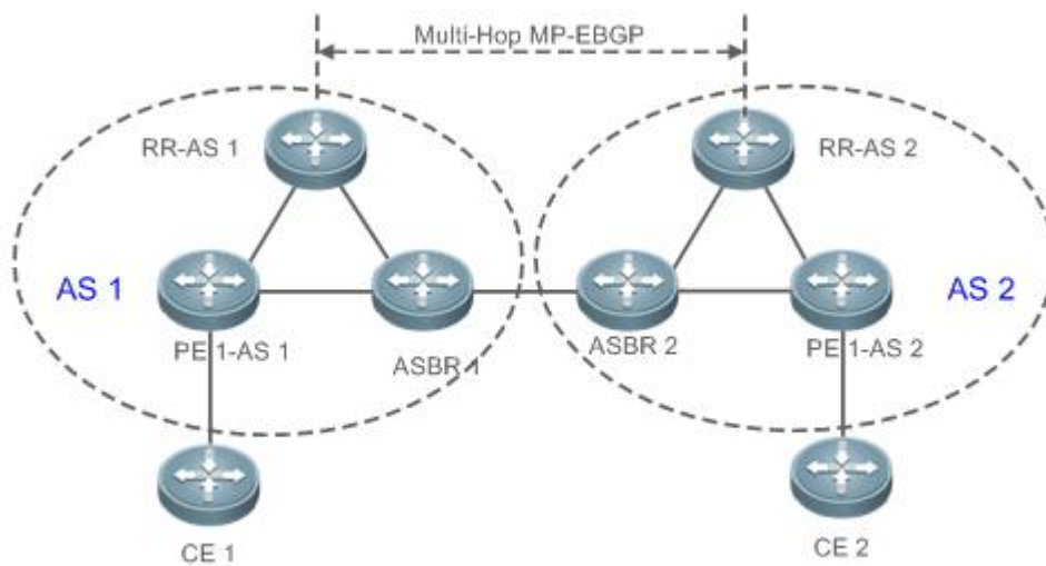
Figure 2-33 Establishment of Inter-RR Multi-hop MP-EBGP for Option C
