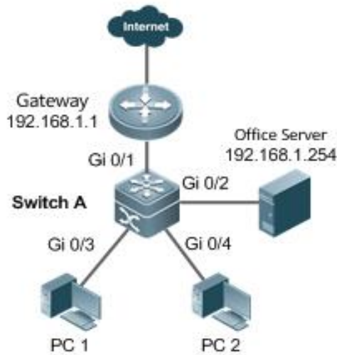
Figure 21-1 Typical Topology of Gateway-targeted ARP Spoofing Prevention
