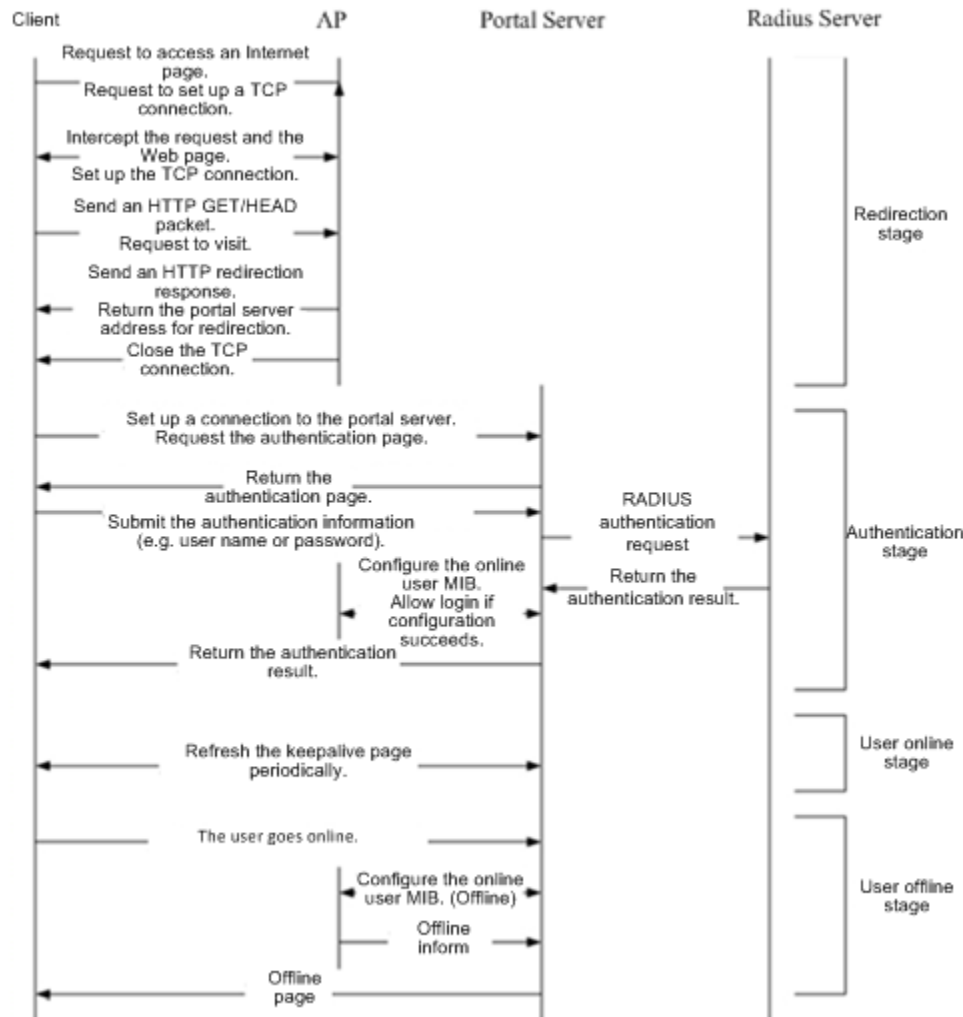
Figure 5-2 Flowchart of Ruijie First-Generation Web Authentication
