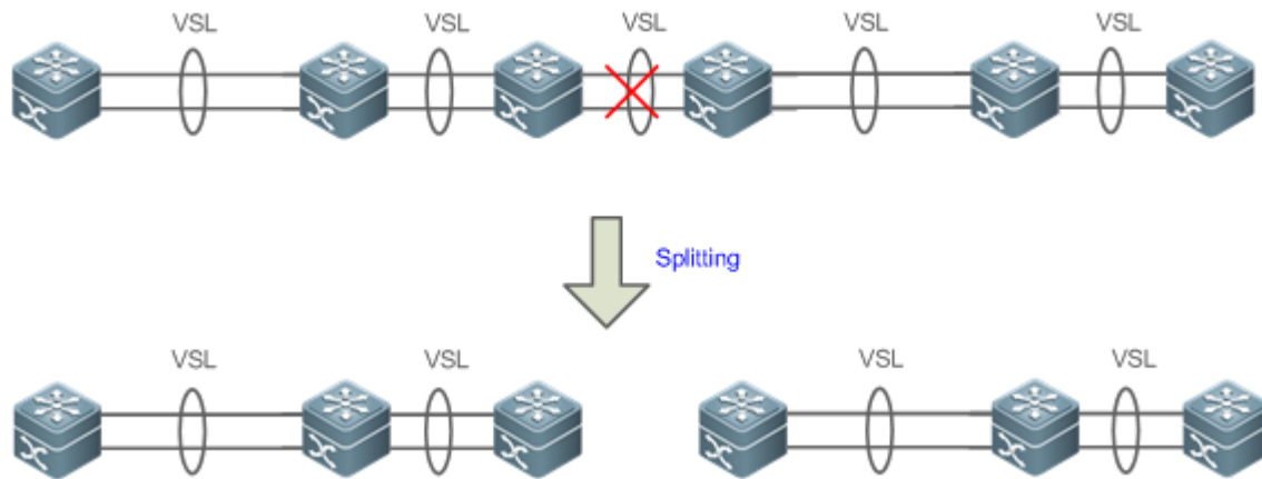
Figure 8-11 Topology splitting
