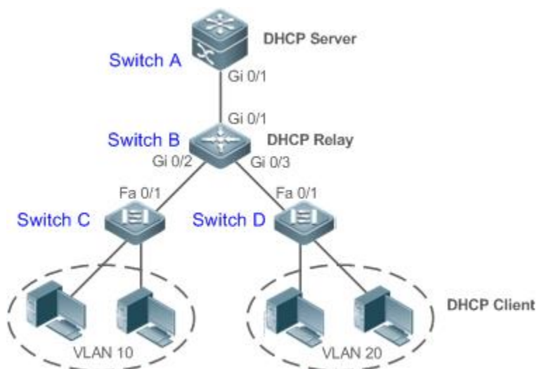
Figure 4-5 DHCP Relay
