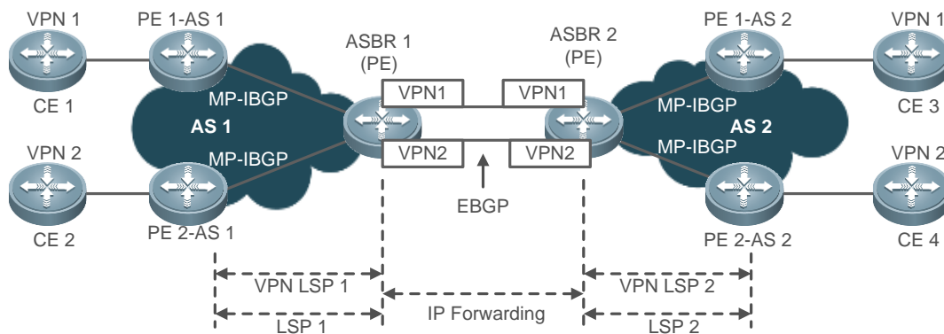
Figure 2-26 VRF-to-VRF Inter-AS VPN
