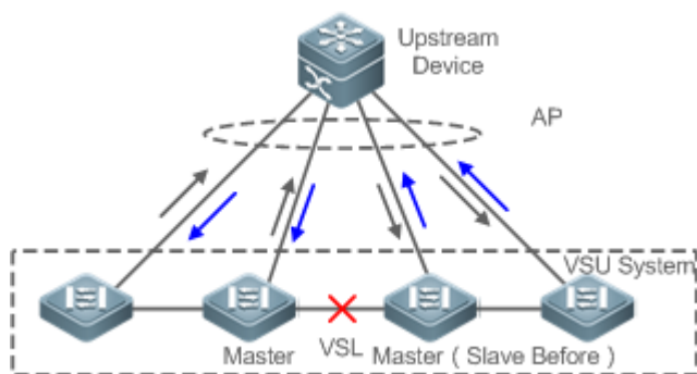
Figure 8-14 MAD based on upstream and downstream devices
