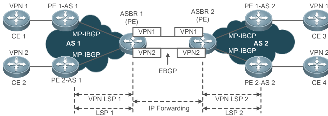
Figure 2-7 VRF-to-VRF Inter-AS VPN
