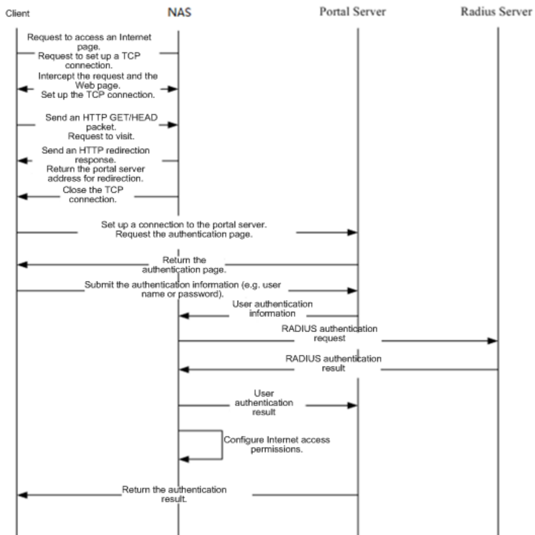
Figure 5-3 Flowchart of Ruijie Second-Generation Web Authentication
