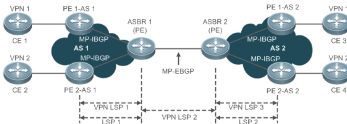
Figure 2-27 Option B Inter-AS VPN
