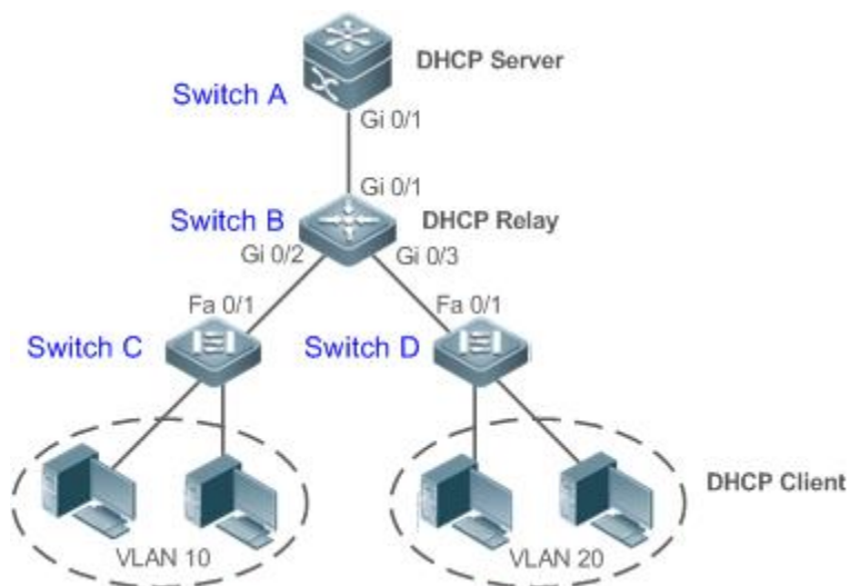
Figure 4-5 DHCP Relay
