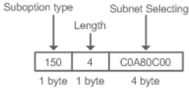
Figure 4-14 Subnet-Selection
