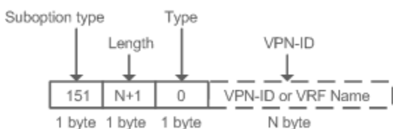
Figure 4-13 VPN-ID
