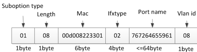
Figure 4-17 Option82-remote-id
