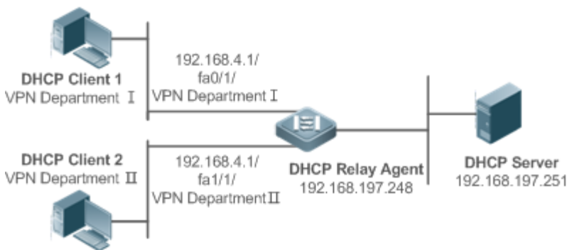
Figure 4-12 Application in MPLS VPN Environment
