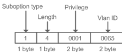
Figure 4-9 Option Format
