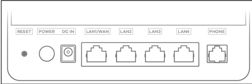
Figure 18 Side Panel (LTE3316-M604)
