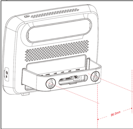
Figure 32 Wall Mounting Screw Specifications
