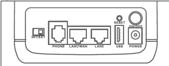
Figure 15 Rear Panel (LTE5388-M804 / LTE5398-M904)
