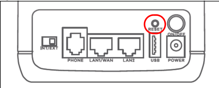
Figure 28 Reset Button (LTE5388-M804 / LTE5398-M904)
