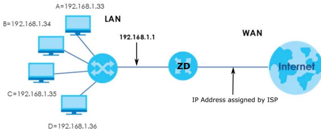
Figure 134 Multiple Servers Behind NAT Example
