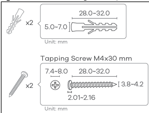
Figure 32 Wall Mounting Screw Specifications
