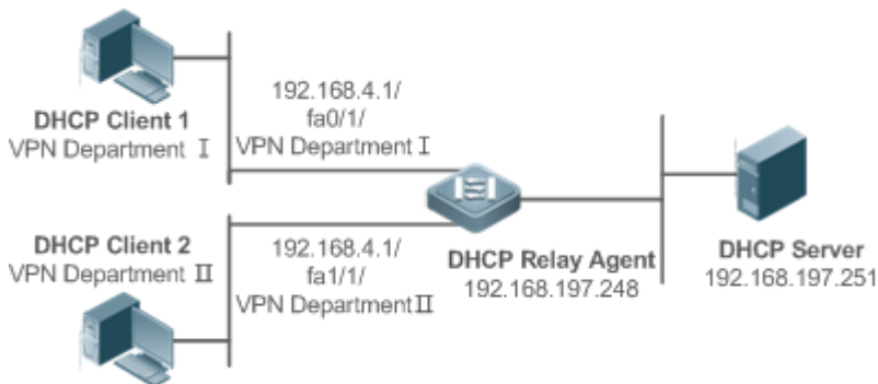
Figure 4-12 Application in MPLS VPN Environment
