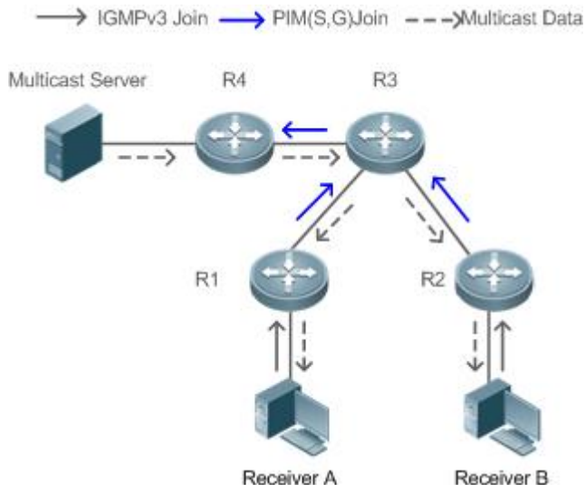
Figure 6-4 SSM Model
