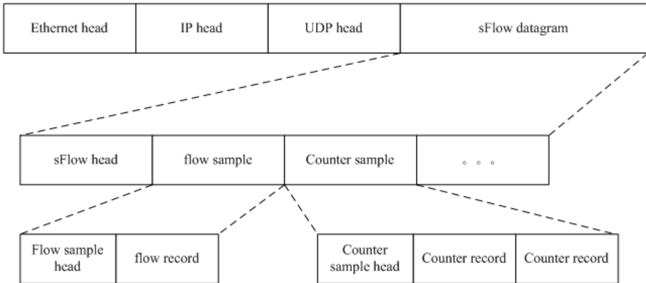
Figure 6-3 sFlow Header
