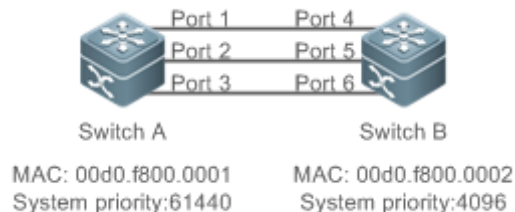
Figure 3-2 LACP Negotiation
