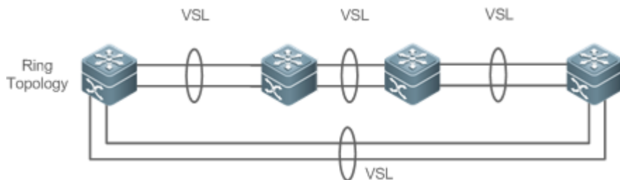
Figure 7-9 Ring Topology
