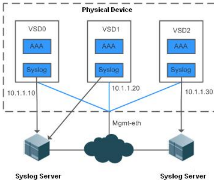
Figure 8-2 Out-of-band Management
