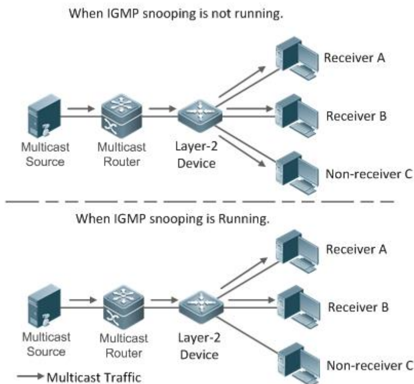
Figure 8-1 Networking Topology of IP Multicast Forwarding within the VLAN Before and After IGMP Snooping Is Run on the Layer-2 Device
