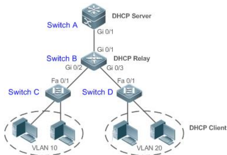
Figure 4-5 DHCP Relay
