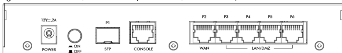
Figure 65 USG FLEX 50/USG FLEX 50W(USG20-VPN / USG20W-VPN) Rear Panel
