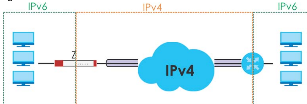
Figure 256 IPv6-in-IPv4 Tunnel
