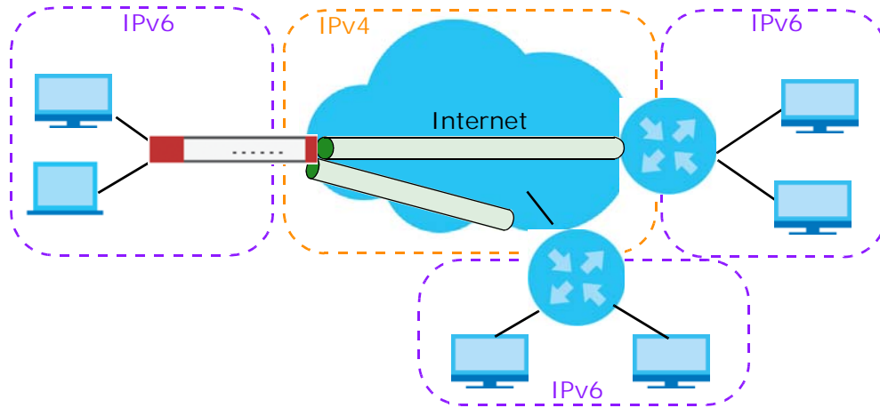
Figure 257 6to4 Tunnel
