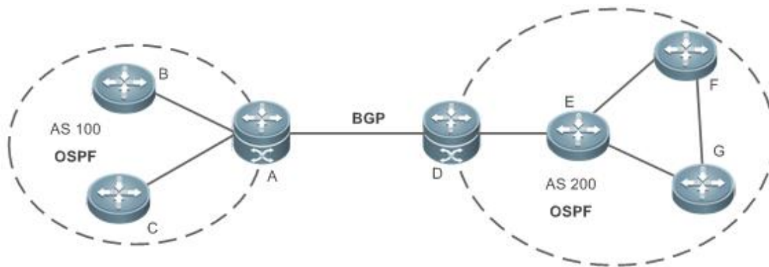
Figure 5-2 Interworking Between OSPF and BGP
