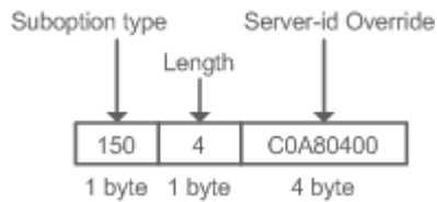
Figure 4-15 Server-Identifier-Override
