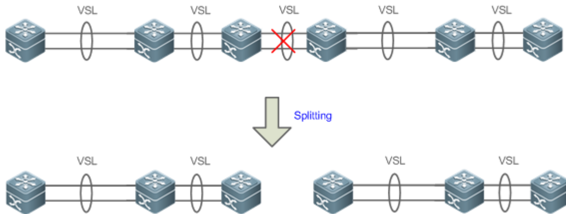
Figure 7-11 Topology splitting
