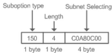
Figure 4-14 Subnet-Selection
