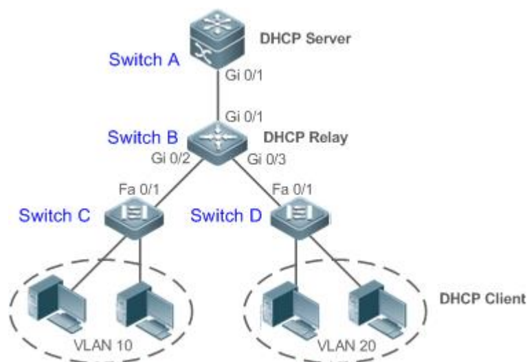
Figure 4-5 DHCP Relay
