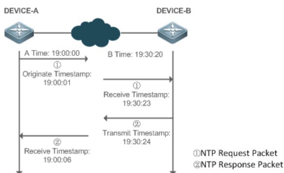
Figure 12-4 Working Principle of NTP
