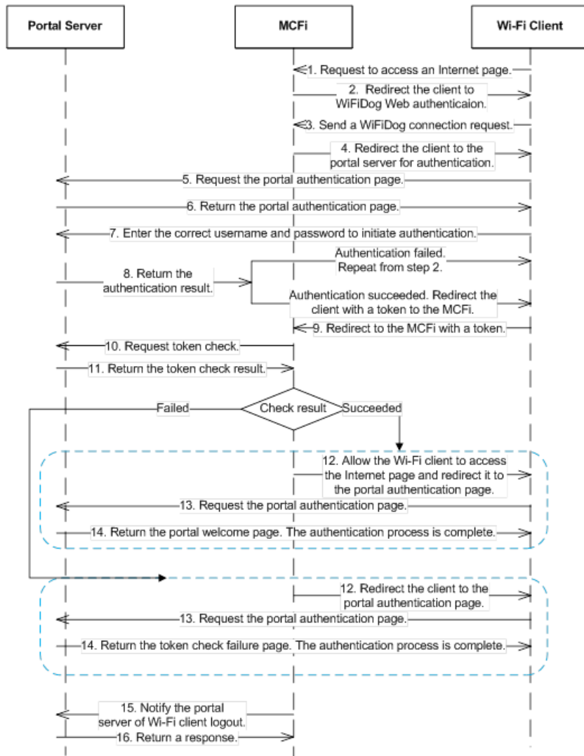
Figure 1-6 Flowchart of WiFiDog Web Authentication
